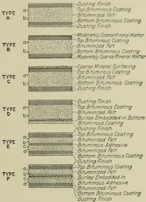
FIG. 199.—Types of Prepared Roofings.
